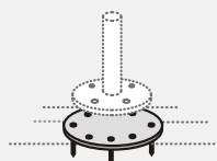
Base Plate 315mm \phi - to bolt to concrete patio or wooden deck
